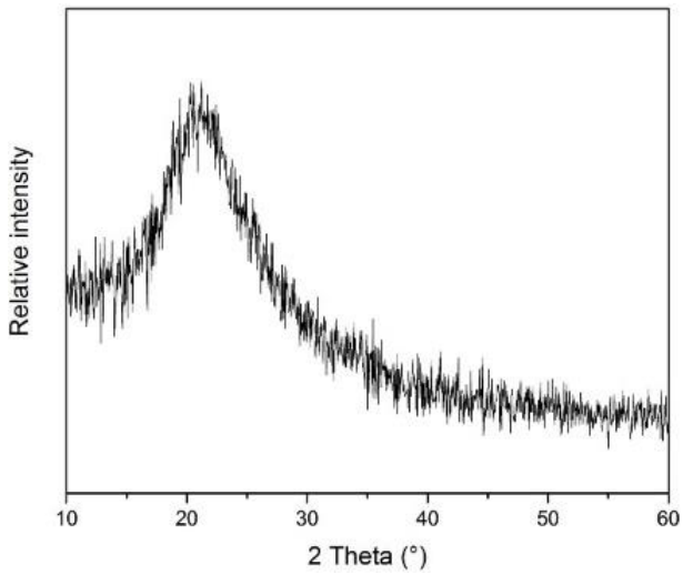
Fig. 1. XRD spectra of as-deposited VO 2 thin films.
