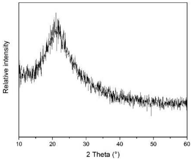
Fig. 3. XRD spectra of as-deposited W-VO 2 thin films.
