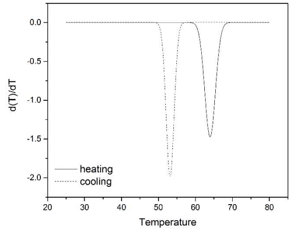
Fig. 6. Gauss fitting derivative logarithmic plots of d(T)/dT - T of the VO 2 thin films annealing at 500 °C.
