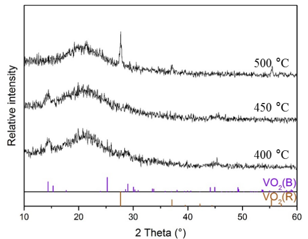
Fig. 4. XRD spectra of W-VO 2 films with varying annealing temperature.
