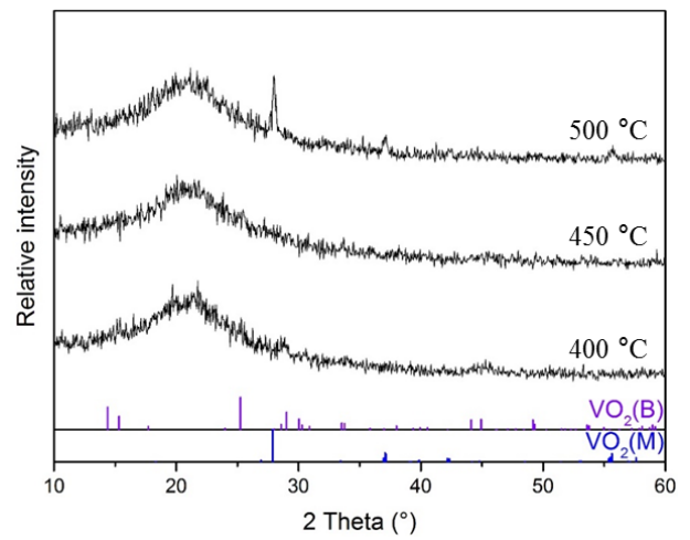
Fig. 2. XRD spectra of VO 2 thin films with varying annealing temperature
