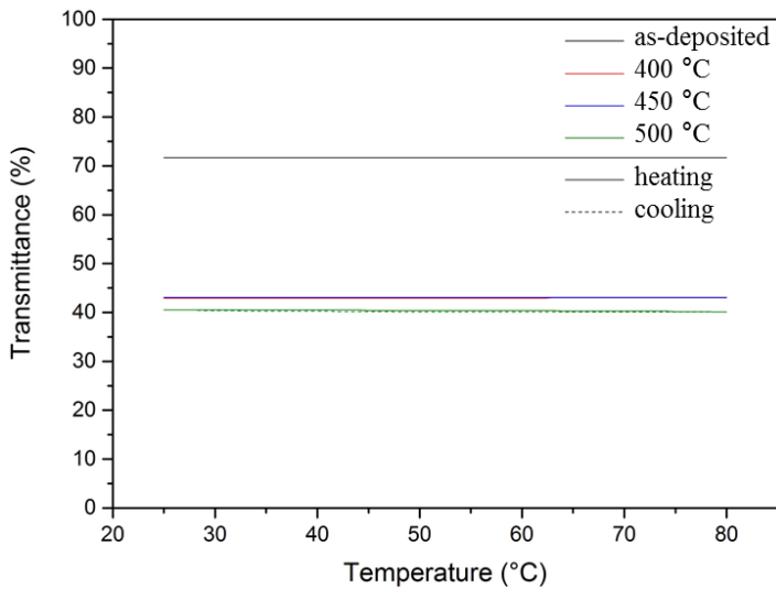
Fig. 7. Transmittance at wavelength 950 nm versus temperature for W-VO 2 thin films with varying annealing temperature.
