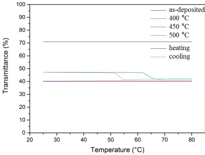
Fig. 5. Transmittance at wavelength 950 nm versus temperature for VO 2 thin films with varying annealing temperature.
