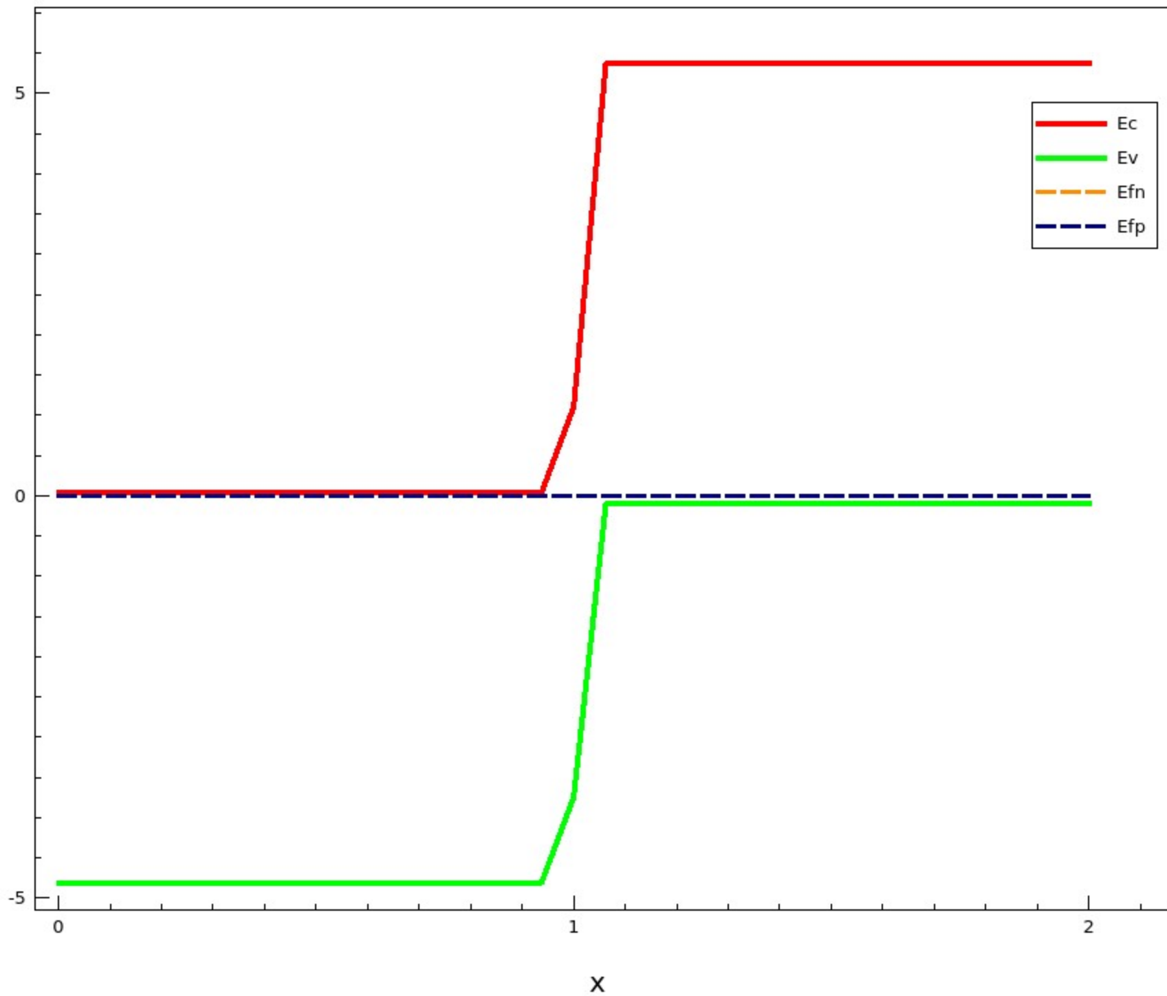
Band Diagram Ga2O3/Diamond
