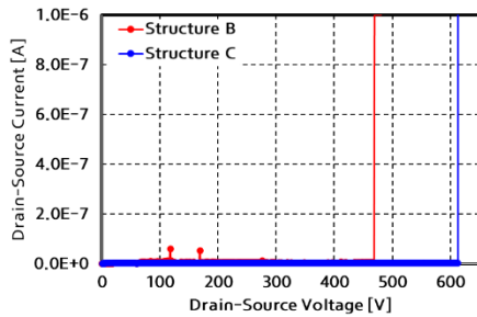
(a) Breakdown Voltage
