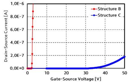
(b) Threshold Voltage
