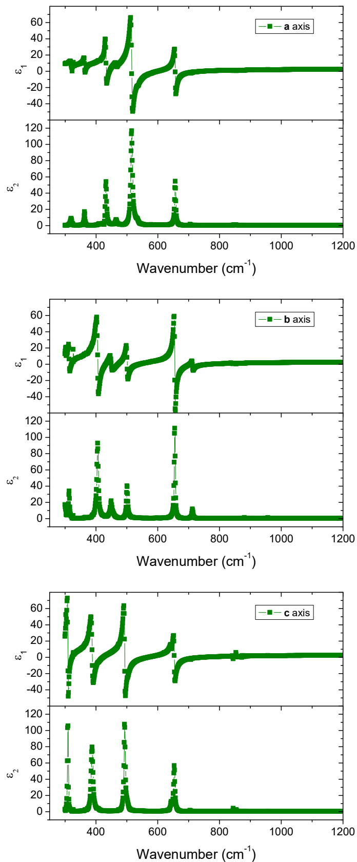
Figure 1: The real and imaginary part of the dielectric tensor function for \text{LiGaO}_2 derived from the point-by-point fit to experimental Mueller matrix data for the mid-infrared spectral range. The dielectric tensor function is shown along crystallographic axes a , b , and c .
