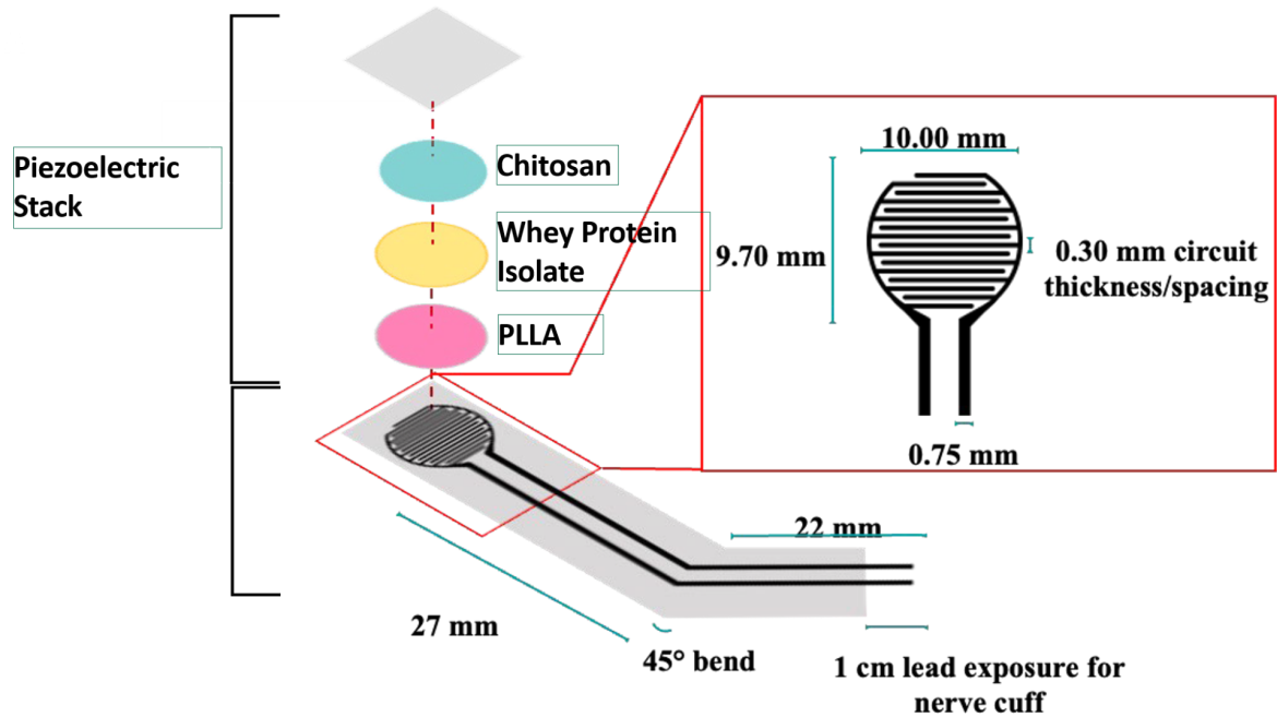
Figure 1. Schematic of piezoelectric implant, with piezoelectric stack in expanded view and dimensions of flexible graphene-based circuitry.
