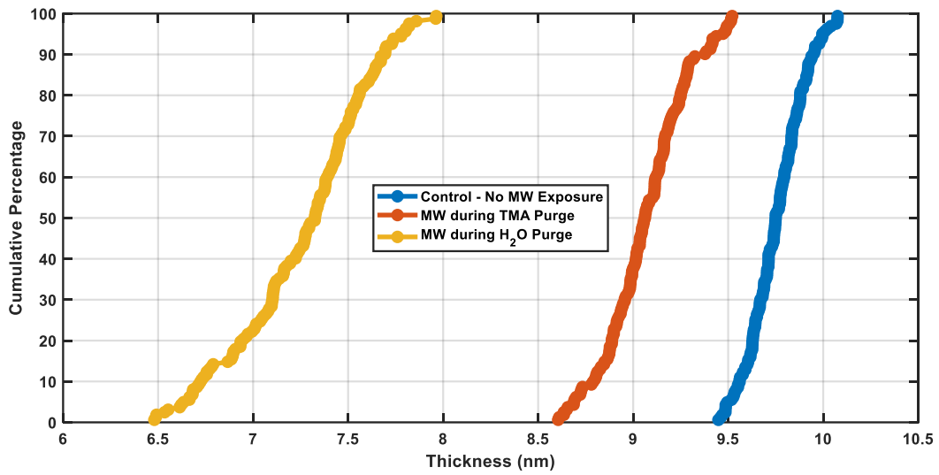
Fig. 1. Cumulative percentage of sites measured vs. Al 2 O 3 film thickness across 150 mm Si wafers, captured using a mapping ellipsometer, for 100 cycle films deposited without (control) and with 30 sec of microwave exposure performed during either the TMA or H 2 O purges of each cycle.
