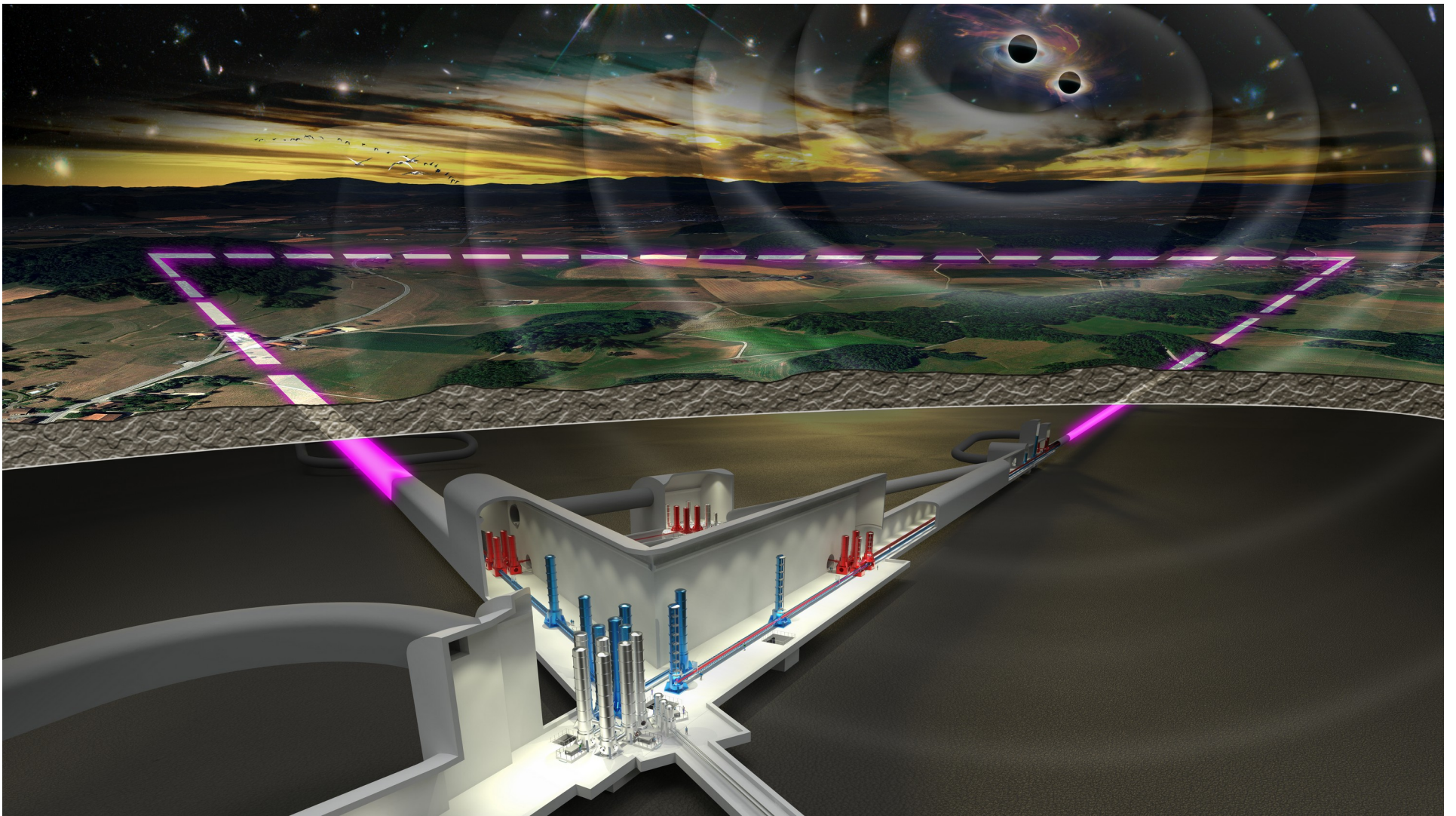
Fig. 1. Artistic impression of the Einstein Telescope, a triangular-shaped underground gravitational wave observatory with 10-km long arms hosting 3 warm and 3 cryogenic interferometers. The total volume of the UHV system exceeds 50,000 m 3 . Courtesy Marco Kraan, Nikhef.
