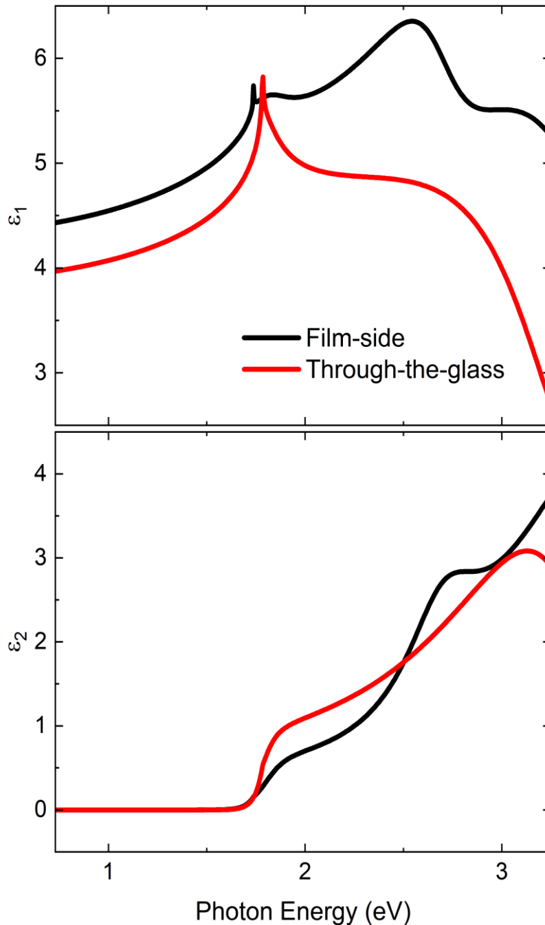
A comparison of dielectric functions of \text{FA}_{0.8}\text{Cs}_{0.2}\text{Pb}(\text{I}_{0.6}\text{Br}_{0.4})_3 when measured in the film-side configuration (black) and through-the glass as a complete device (red).
