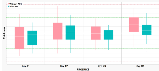
Control simulation result of APC system by product
