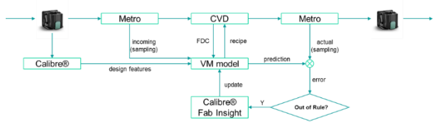
Schematic diagram of APC system
