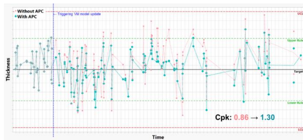
Control simulation result of APC system
