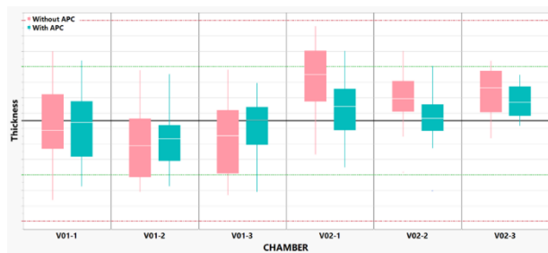
Control simulation result of APC system by chamber
