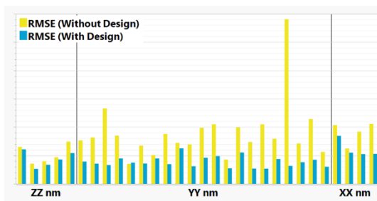
Segmented comparison of the VM model with and without design features by product
