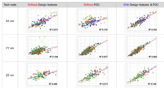
VM modeling with and without incorporating design features and FDC data
