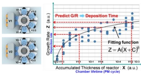
PM cycle and chamber-to-chamber film growth rate variations
