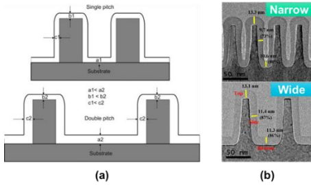
(a) schematic of the difference in film thickness for a single and double pitch (b) TEM images of silicon nitride film thickness differences between a wide and a narrow pattern
