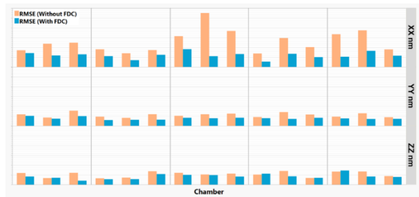
Segmented comparison of the VM model with and without FDC by chamber
