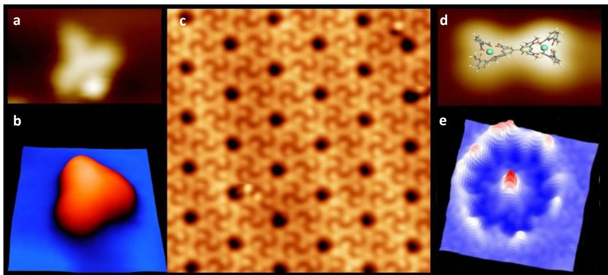
Figure. STM images and spectroscopic maps of Eu based molecular complexes on Au(111). (a) [\text{Eu}(\text{pcam})_3]^{3+} (Europium(III) tris(2,6-pyridinedicarboxamide)) with triflate ( \text{CF}_3\text{SO}_3^- ) counter ion attached, (b) without the counter ion, (c) 2-D self-assembled layer formed by Ullmann coupled \text{Eu}(\text{pcam})_3 , (d) coupled \text{Eu}(\text{pcam})_3 and (e) spectroscopic map of a self-assembled structure at -200mV.
