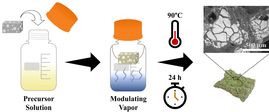
Schematic diagram of sorption-vapor synthesis leading to a plant fiber sponge@UiO-66-NH 2 composite.
