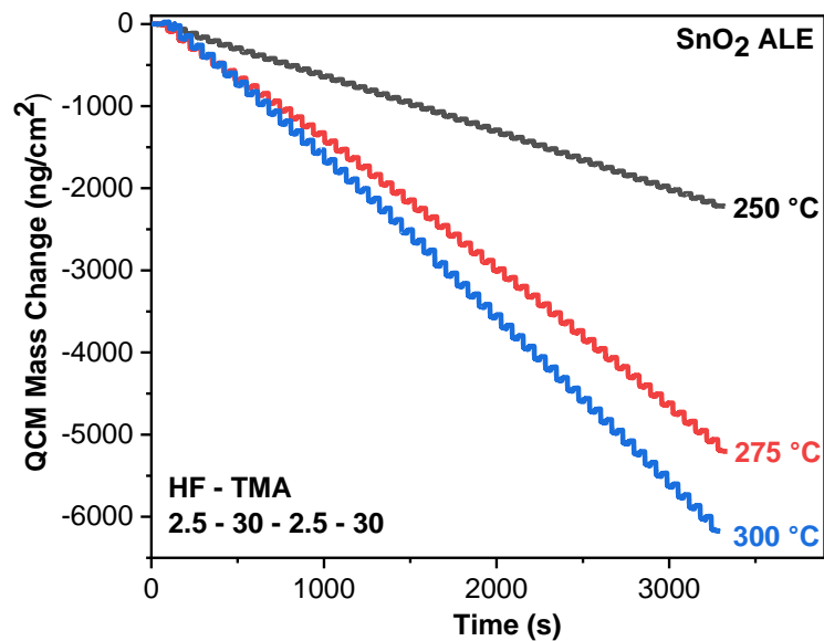
Supplemental Figure 1. QCM mass change vs time showing 50 SnO 2 ALE cycles using HF and TMA at 250, 275 and 300 °C.
