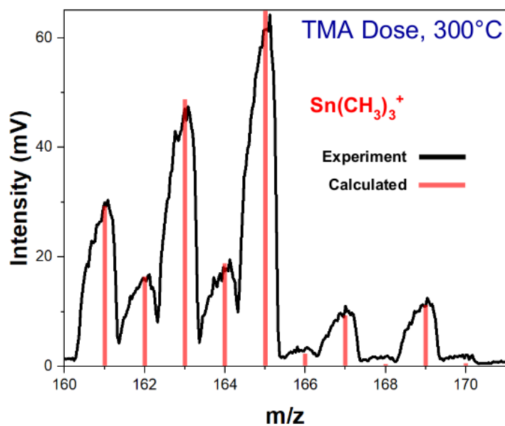
Supplemental Figure 2. Mass spectrum showing ion signals for Sn(CH 3 ) 3 + from TMA dose during HF-TMA cycles on SnO 2 at 300 °C.
