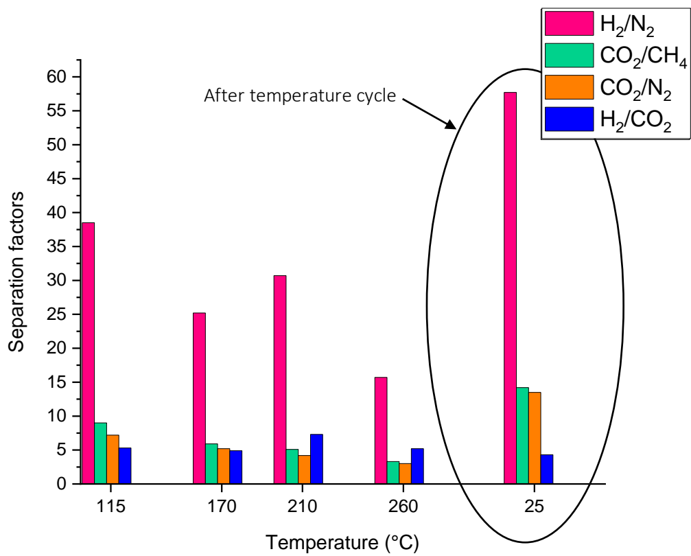
Figure 2: Influence of the temperature working condition on a 500 MLD cycles alucone membrane post-treated at 300^\circ\text{C} for 2h under \text{N}_2 atmosphere (error)
