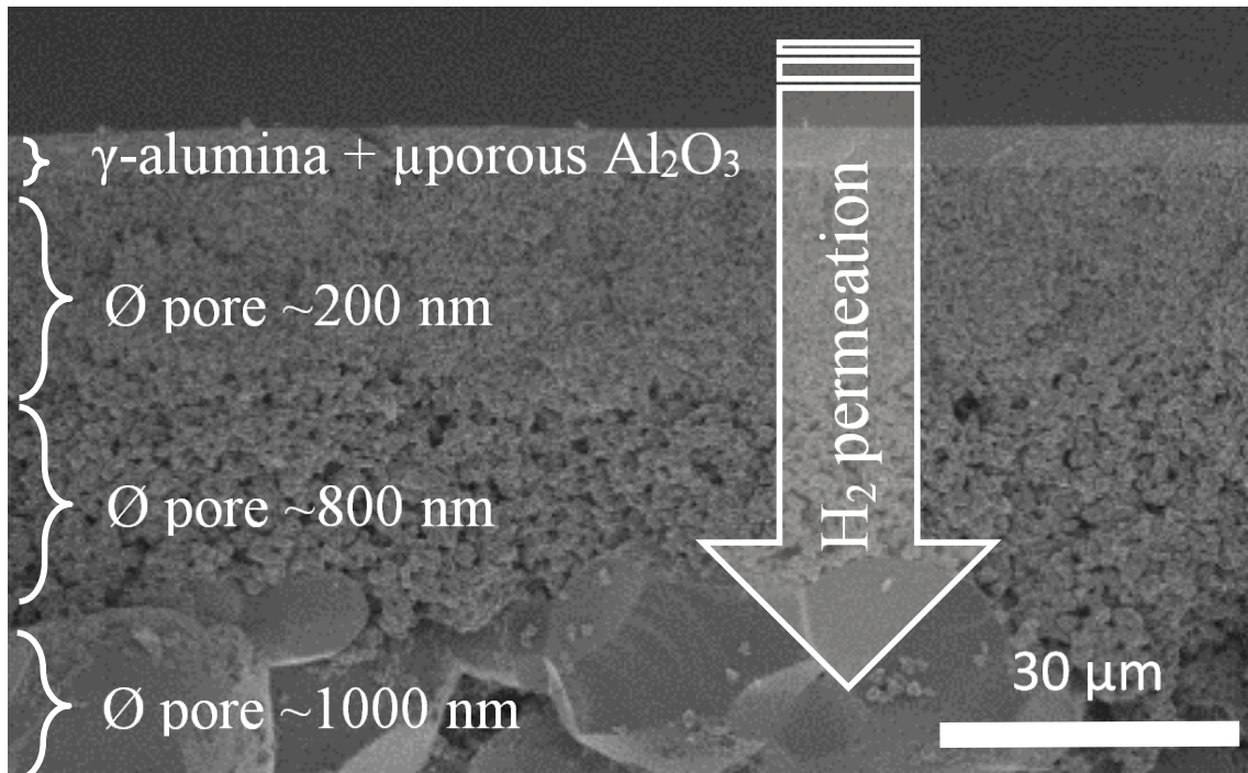
Figure 1: SEM image of ceramic membrane cross-section showing the membrane top-layer on asymmetric support
