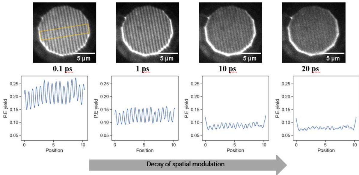
Upper panel: PEEM images of an InP platelet at different pump-probe delays (0.1 ps, 1 ps, 10 ps, and 20 ps). The intensity profile of the spatial modulation, averaged along the yellow rectangle is shown in the lower panel.
