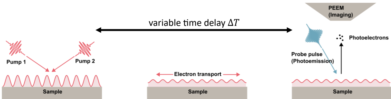
Schematic with the principle of transient grating time-resolved PEEM
