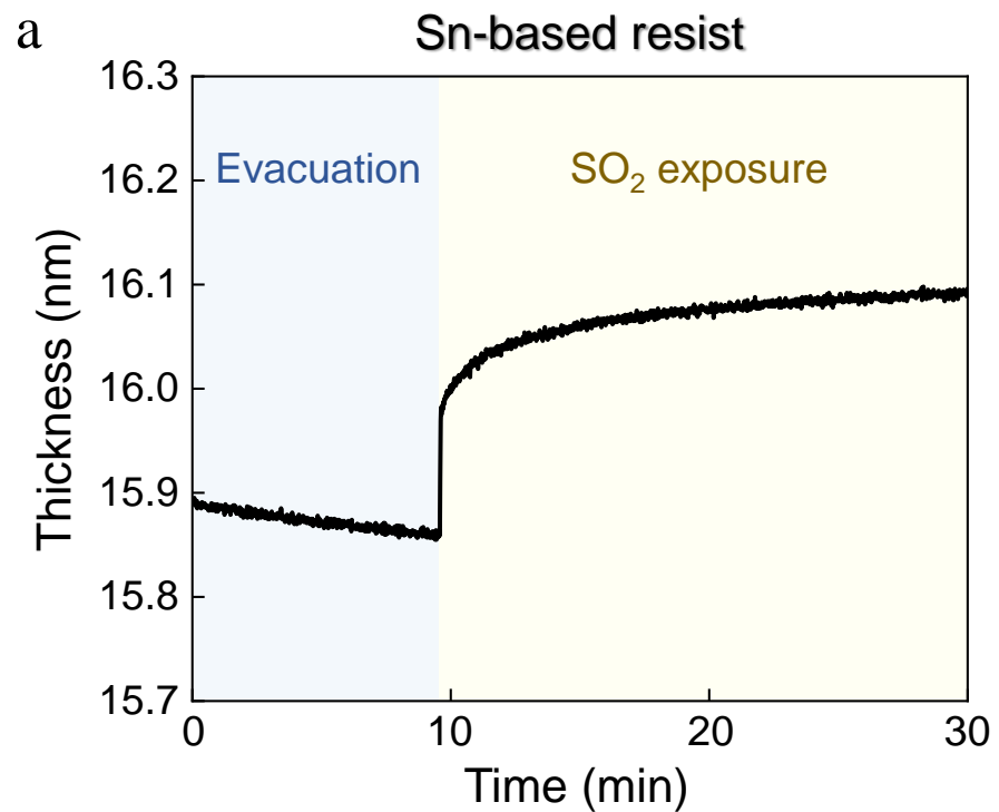
Figure S1. Selective physisorption of SO 2 to (a) Sn-based resist and (b) SiO 2 .
