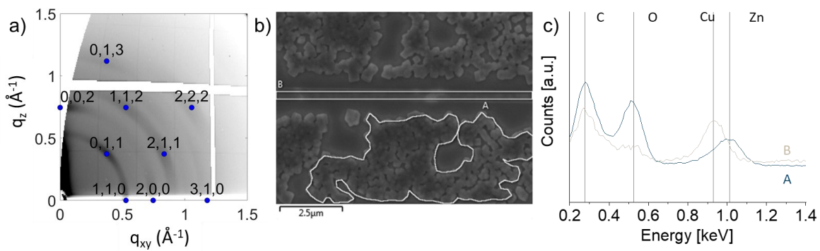
Molecular layer deposition of ZIF-8 on self-assembled monolayers a) Synchrotron grazing incidence XRD showing preferential crystalline orientation, b) Scanning electron microscopy illustrating the area selectivity, and c) EDX spectra from selected areas indicated in panel b.
