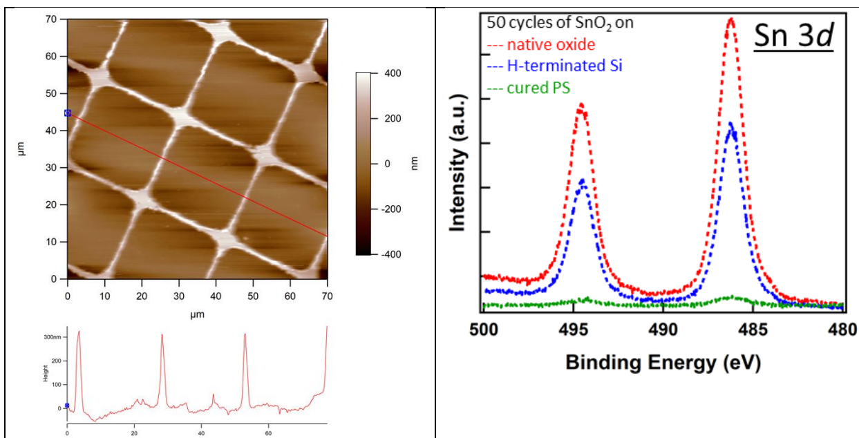
Figure 1. AFM image of 20 cycles of SnO 2 grid patterns after 30 s of SF 6 RIE etching at room temperature and 200 mTorr
