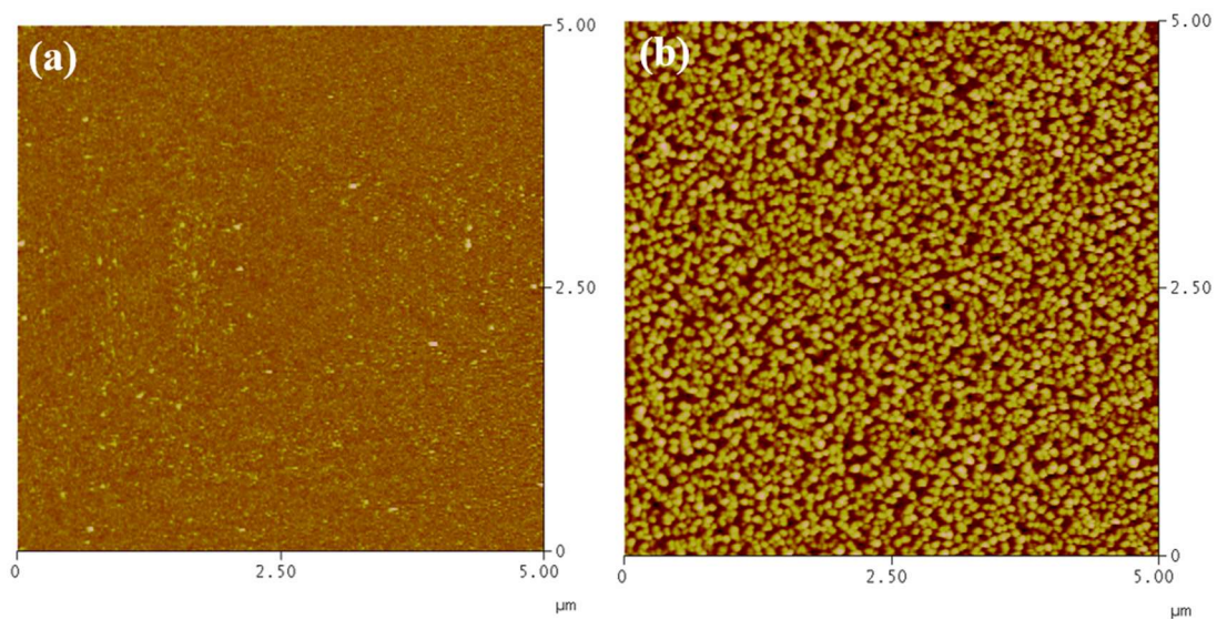
Fig. 1. AFM images of (a) as-deposited and (b) annealed (\text{SiC})_{63.6}\text{V}_{36.4} film.
