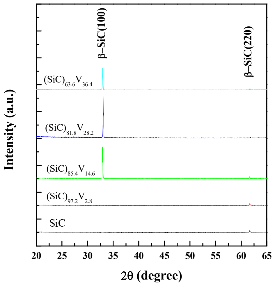
Fig. 2. XRD spectra of SiC and various V-doped SiC films after 1000 °C annealed.
