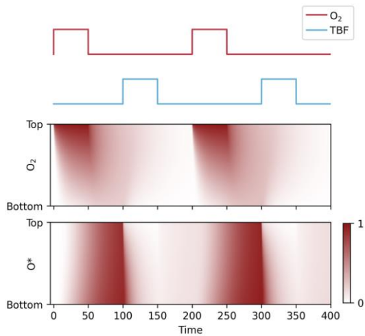
Fig. 1: Simulated concentration profiles of oxygen reservoirs in the \text{Fe}_2\text{O}_3 film. \text{O}_2 diffuses to the bottom, where the Pt substrate can activate it. The activated oxygen diffuses back to the top where it becomes available for consumption by TBF (or possibly another precursor).
