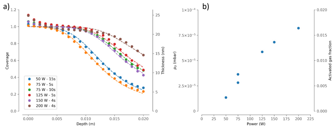
Fig.1: a) fit of simulated depth profiles to real-world data obtained for various plasma conditions. b) obtained partial pressures as a function of plasma power from these data.
