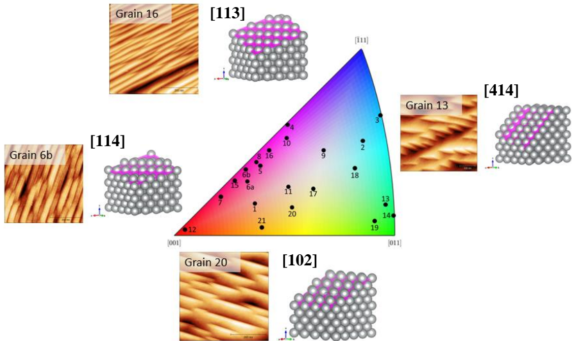
Figure 1: Stereographic triangle with surface grain orientations as they are distributed in the Ni-11Cr-6Mo sample. STM images were taken at 500 x 500 nm after annealing in UHV. VESTA crystal structures corresponding to the Z direction of each grain are shown next to their corresponding STM images, with Miller indices noted in the figure.
