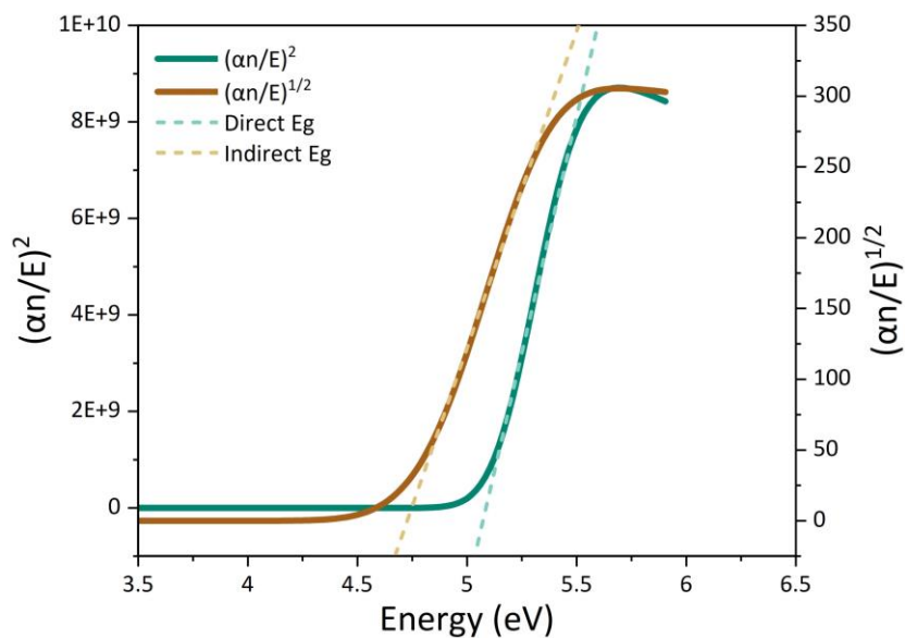
Figure 1: Direct and Indirect optical bandgaps of Zinc gallate thin films determined using a modified Cody formalism
