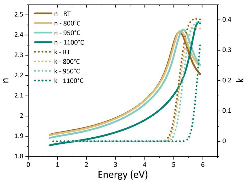
Figure 2: Optical constants of Zinc gallate thin films at room temperature and different annealed temperatures
