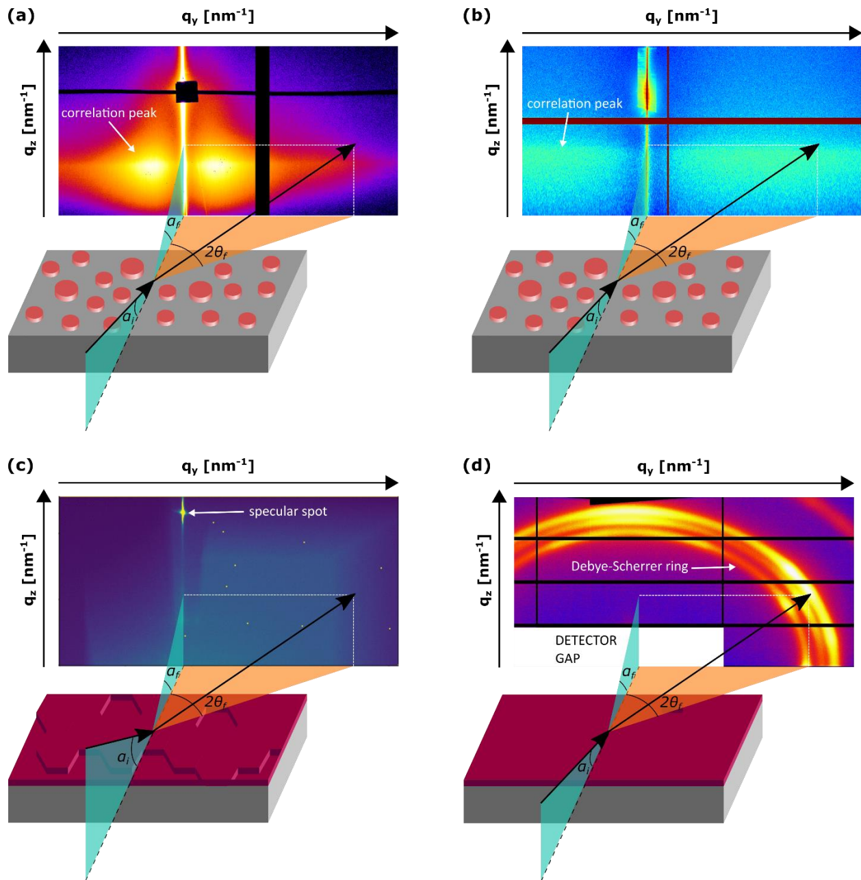
Figure 1. Experimental geometry for study of (a) island growth using GISAXS, (b) island growth using GISAXS with highly coherent x-ray beam, (c) layer-by-layer growth using scattering at greater incident angles, and (d) ultrathin film crystal structure and orientation using GIWAXS.
