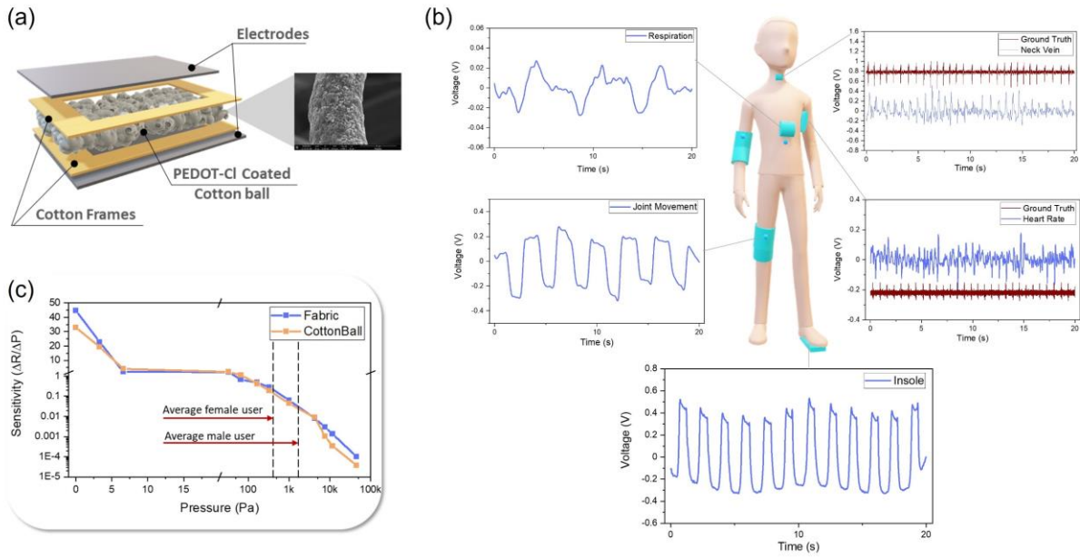
Figure 1- a) Schematic illustration of the sensor including the SEM image of the PEDOT-Cl coated layer, b) Physiological and body movements signals acquired via sensor, c) Sensitivity of the sensor over a wide range of pressures
