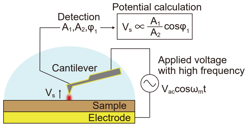
Fig. 1 Experimental setup of OL-EPM
