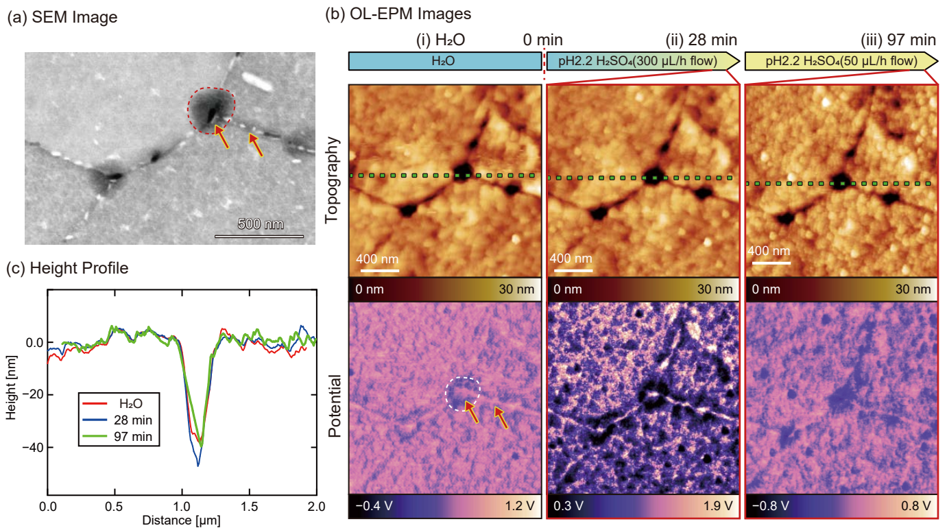
Fig. 2 (a) SEM image at the GB. (b) Time-lapse images of topography and potential at the GB in sulfuric acid obtained by OL-EPM. (c) Height profile at the GB.
