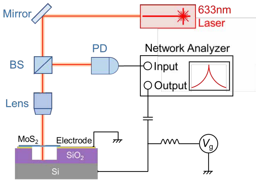
Fig. 1 Measurement setup.
