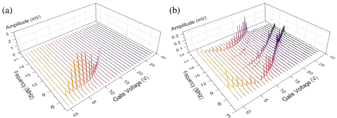
Fig. 3 3D color plot of the resonant response of the device with gate voltage increase (a) and gate voltage decrease (b) , respectively
