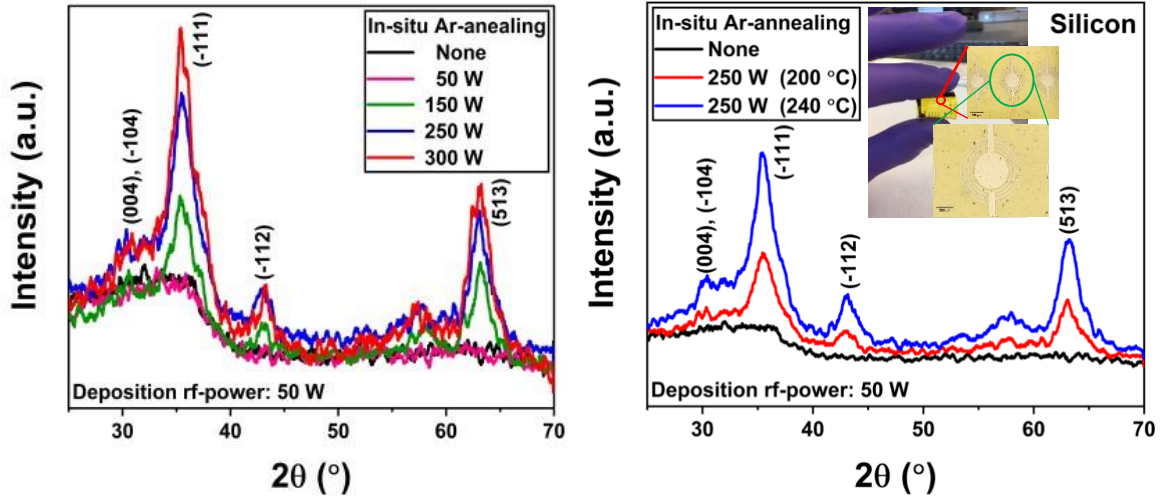
Figure 1. GIXRD spectra of 300-cycle grown \text{Ga}_2\text{O}_3 films at 50 W (a) with varying in-situ Ar-annealing plasma powers. (b) at 250 W in-situ Ar-annealing power as a function of changing substrate temperature. Inset in (b) shows a proof-of-concept inter-digitated device structures fabricated by growing \text{Ga}_2\text{O}_3 as an active layer on Kapton flexible substrate.
