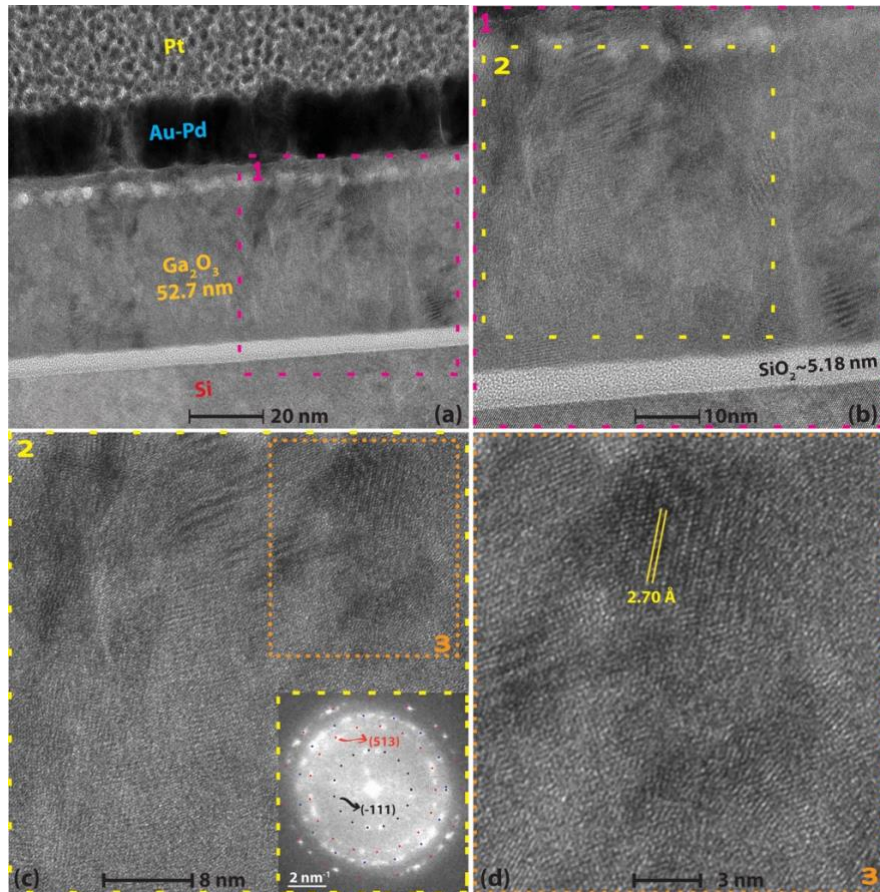
Figure 2. (a) HR-TEM micrographs of 500-cycle \text{Ga}_2\text{O}_3 sample grown at 240 °C substrate temperature with 50 W Ar/ \text{O}_2 plasma and 250 W in situ Ar-plasma annealing. (b) Zoomed-in image over the selected region #1 as drawn in (a) showing several randomly oriented crystal domains. (c) Close-up view of HR-TEM scan over the selected region #2 as depicted in (b) along with its Fast Fourier Transform (FFT) as an inset, displaying ring-like patterns of the polycrystalline film structure. (d) Magnified HR-TEM micrograph over the smaller region #3 as shown in (c), further revealing the high-resolution lattice features of \text{Ga}_2\text{O}_3 sample.
