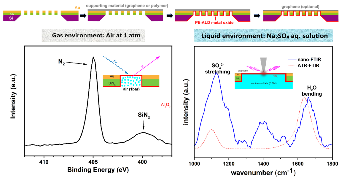
Fabrication process of ultra-thin free-standing oxide membrane and the application on High pressure XPS (1 bar) and nano-FTIR.
