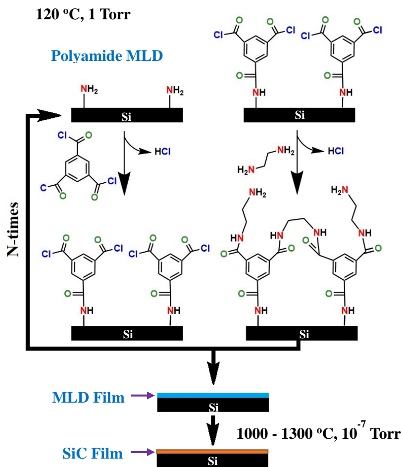
Figure 1. Overall approach to SiC film synthesis by heat treatment of MLD polyamide film on Si
