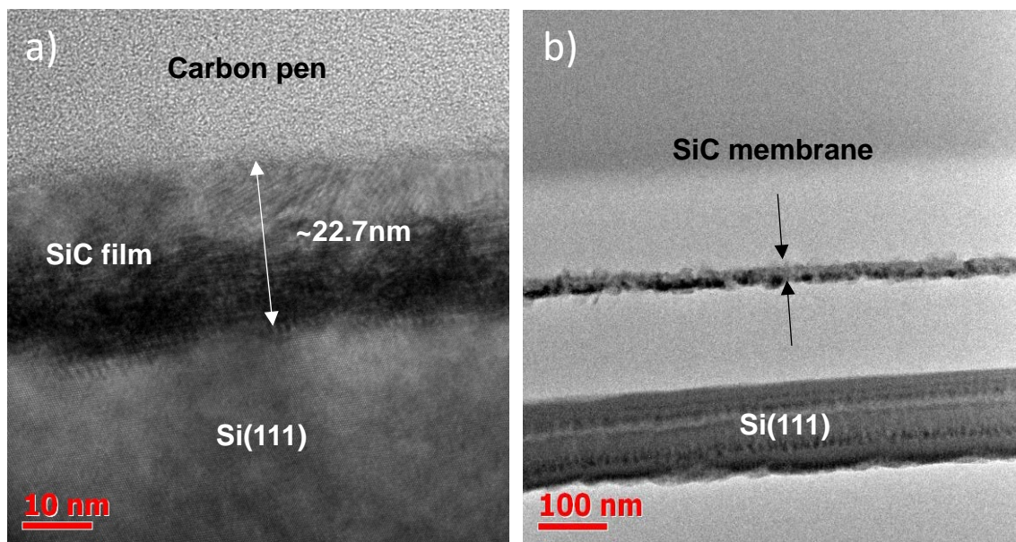
Figure 2. Cross-sectional TEM images of a) thin SiC film synthesized on Si(111) substrate, b) suspended SiC thin film membrane formed by Si sublimation
