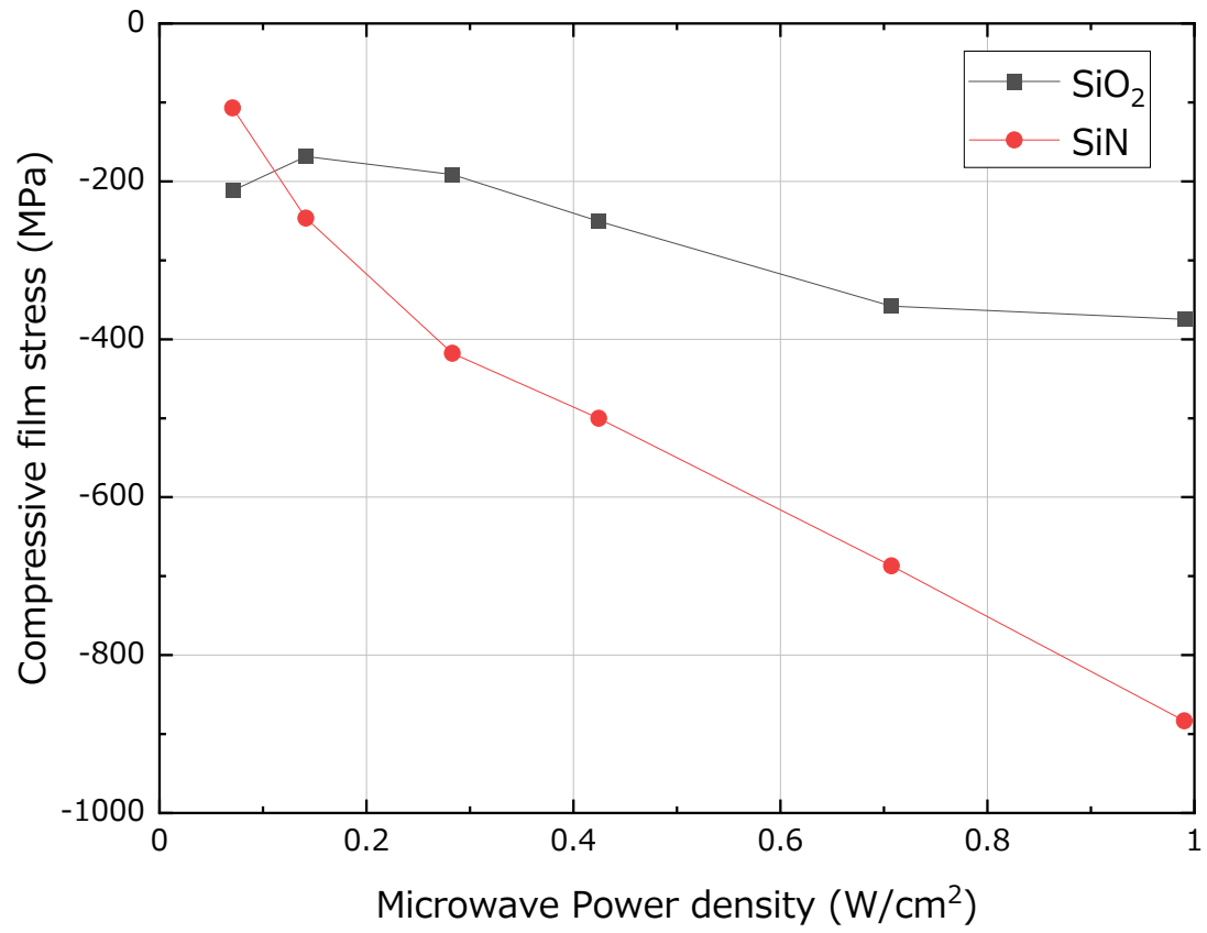
Fig. Microwave power density dependence of film stress in SiO 2 and Si 3 N 4 films
