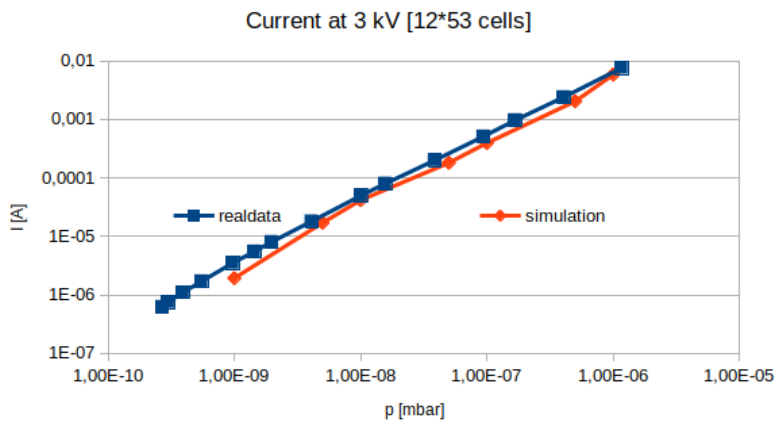
Fig. 2: current-pressure curve of an 800 l/s ion pump with N 2 background gas
