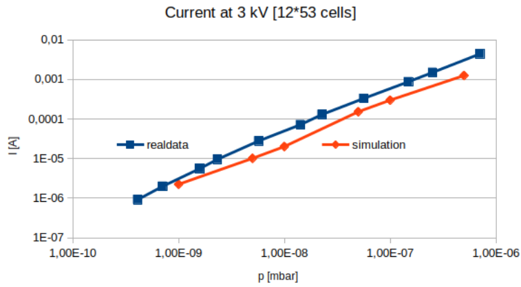
Fig. 1: current-pressure curve of an 800 l/s ion pump with H 2 background gas
