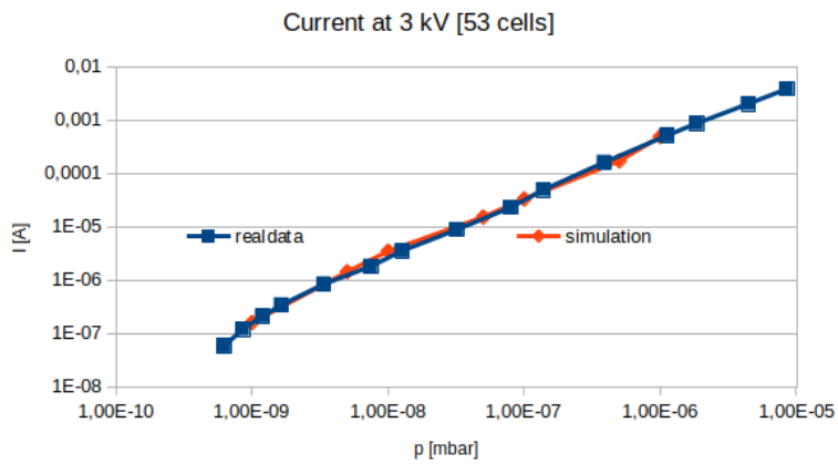
Fig. 3: current-pressure curve of a 40 l/s ion pump with N 2 background gas
