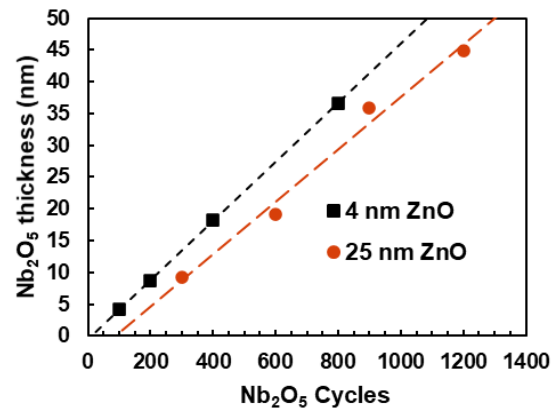
Figure 2. Nb 2 O 5 thickness vs Nb 2 O 5 ALD cycles on 4 nm ZnO (black squares) and 25 nm ZnO (orange circles). Dashed lines indicate linear fits for determining GPC and nucleation cycles.
