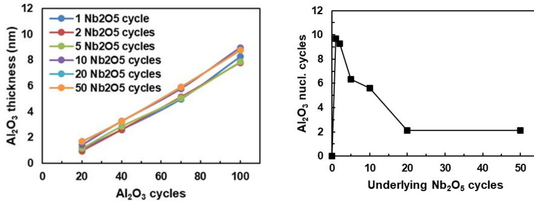
Figure 1. (Left) Plot of Al 2 O 3 thickness versus Al 2 O 3 ALD cycles for different underlying Nb 2 O 5 cycles. (Right) Plot of Al 2 O 3 nucleation cycles vs underlying fixed Nb 2 O 5 cycles..
