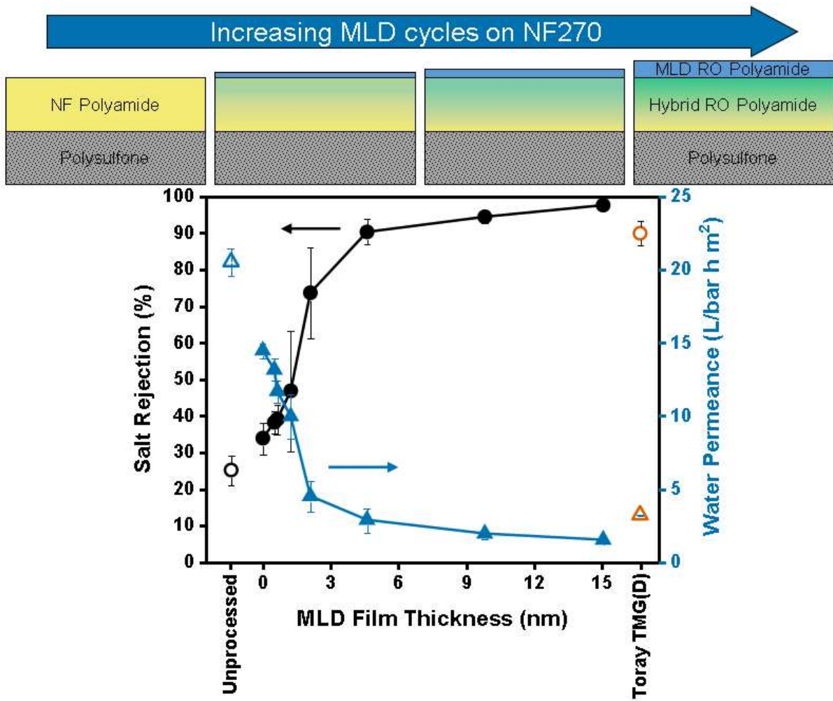
Figure 1. Desalination results for RO samples and NF270 samples modified with MLD versus number of MLD film thickness. Spatial MLD was performed in a rotating cylindrical drum at 20 RPM and 115°C.
