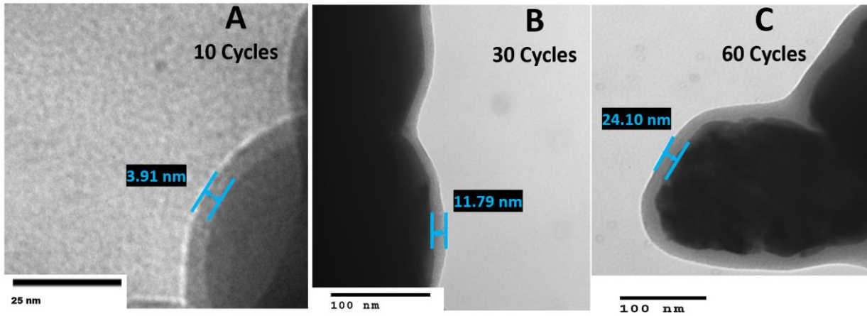
Figure 1. Polyamide films deposited by MLD on ZrO_2 nanoparticles. Depositions were performed at 67 °C with adipoyl chloride and ethylene diamine and showed a growth rate of 4 Å/cycle. A) 10 cycles, B) 30 cycles and C) 60 cycles of polyamide MLD are shown here.
