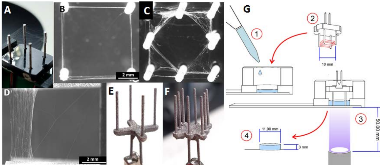
Figure. (A) Fiber array suspended on 4-pillar electrode (B) Top-down view fiber array (C) Top-down view fiber array on 8-pillar electrode (D) Side view of 4 pillar array (E) 4-pillar (F) 8-pillar (G) Schematic for the encapsulation of fiber array in GGMA.
