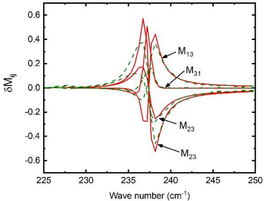
Fig. 2 Off-diagonal elements of the Mueller matrix of OHE in GaSb at 300 K. Red (solid) model and green (dashed) experimental.
