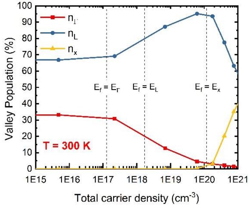
Fig. 1 Distribution of the total electron density in different valleys of GaSb at 300 K.
