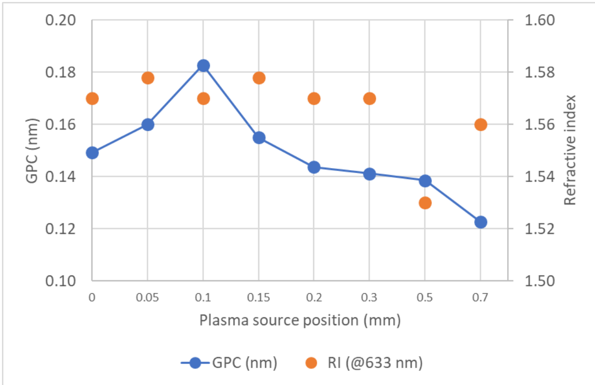
Fig. 1 GPC and refractive index of deposited alumina as function of plasma source position
