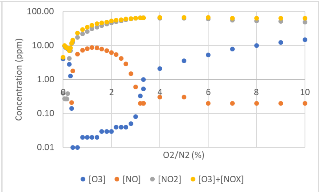
Fig.2 Exhaust gas composition as function of percentage oxygen in plasma gas
