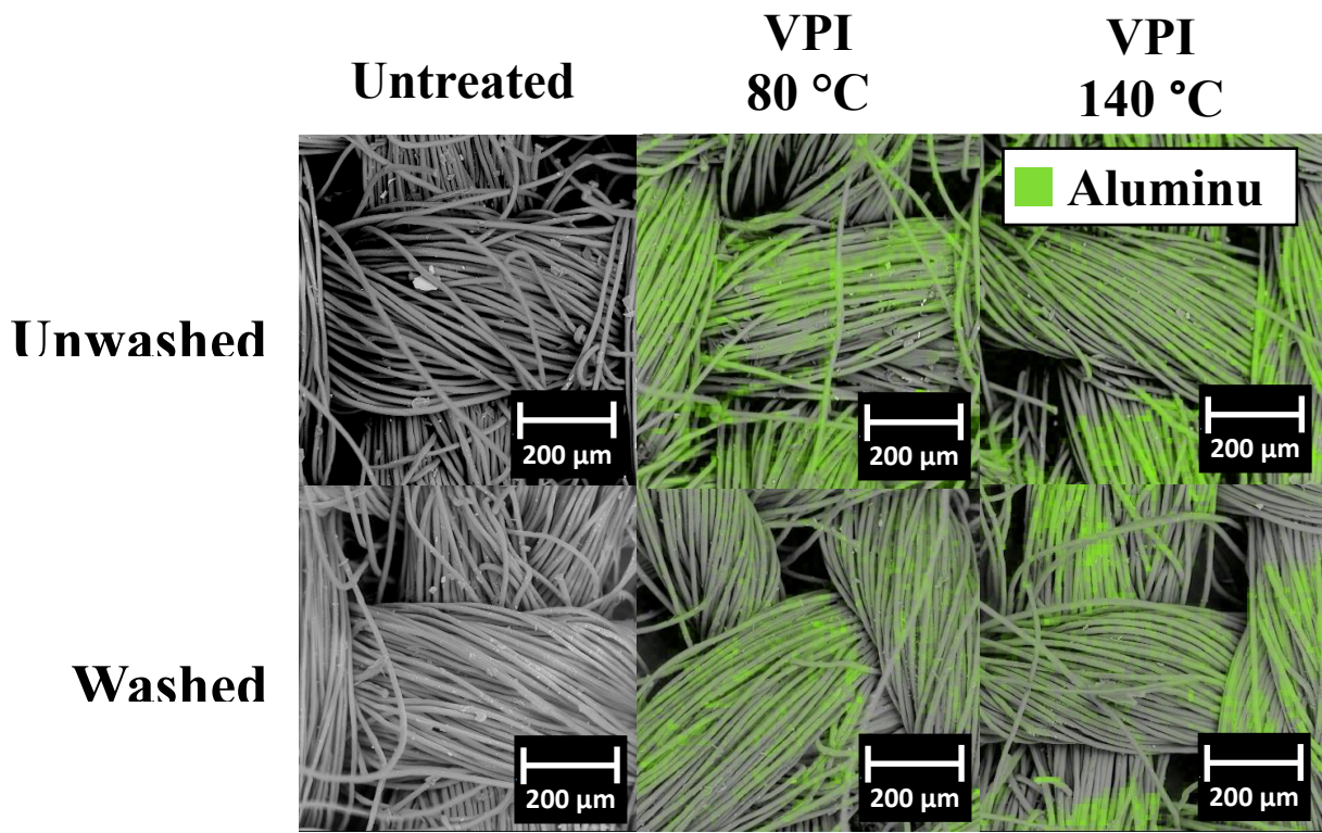
Figure 2. Elemental mapping of infiltrated fabrics collected with SEM/EDX confirming the presence of aluminum in washed fabrics.
