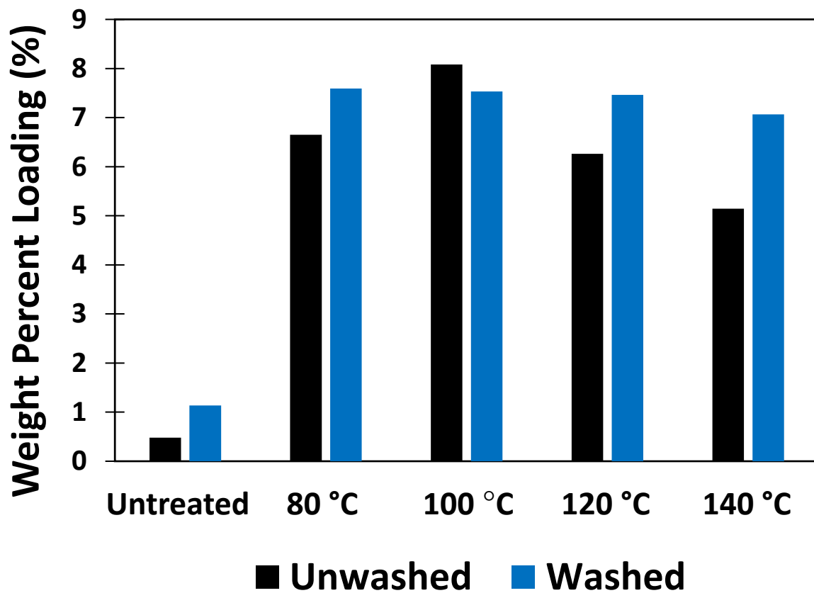
Figure 1. The inorganic loading in vapor phase infiltrated polyester fabrics is retained after washing in DI water at 100°C for 90 minutes, as shown from the results of thermogravimetric analysis.
