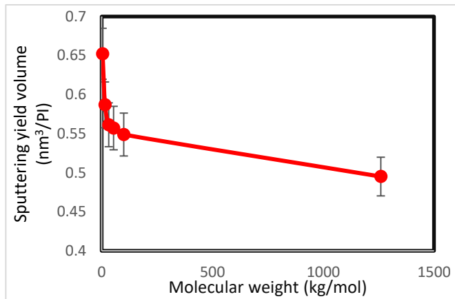
Figure 1. Sputtering yield volume as function of molecular weight of PMMA thin films sputtered by 500eV Cs +
