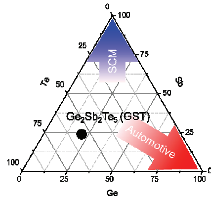
Figure 2 : Ge-Sb-Te phase-change material ternary diagram associated to targeted applications.
