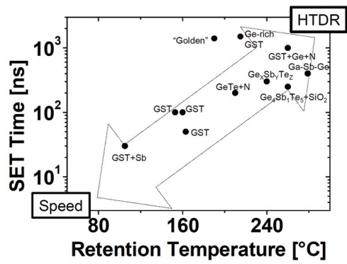
Figure 1 : SET Time vs Retention Temperature for different phase-change materials. A trade-off exists between high-temperature data retention and SET programming time.
