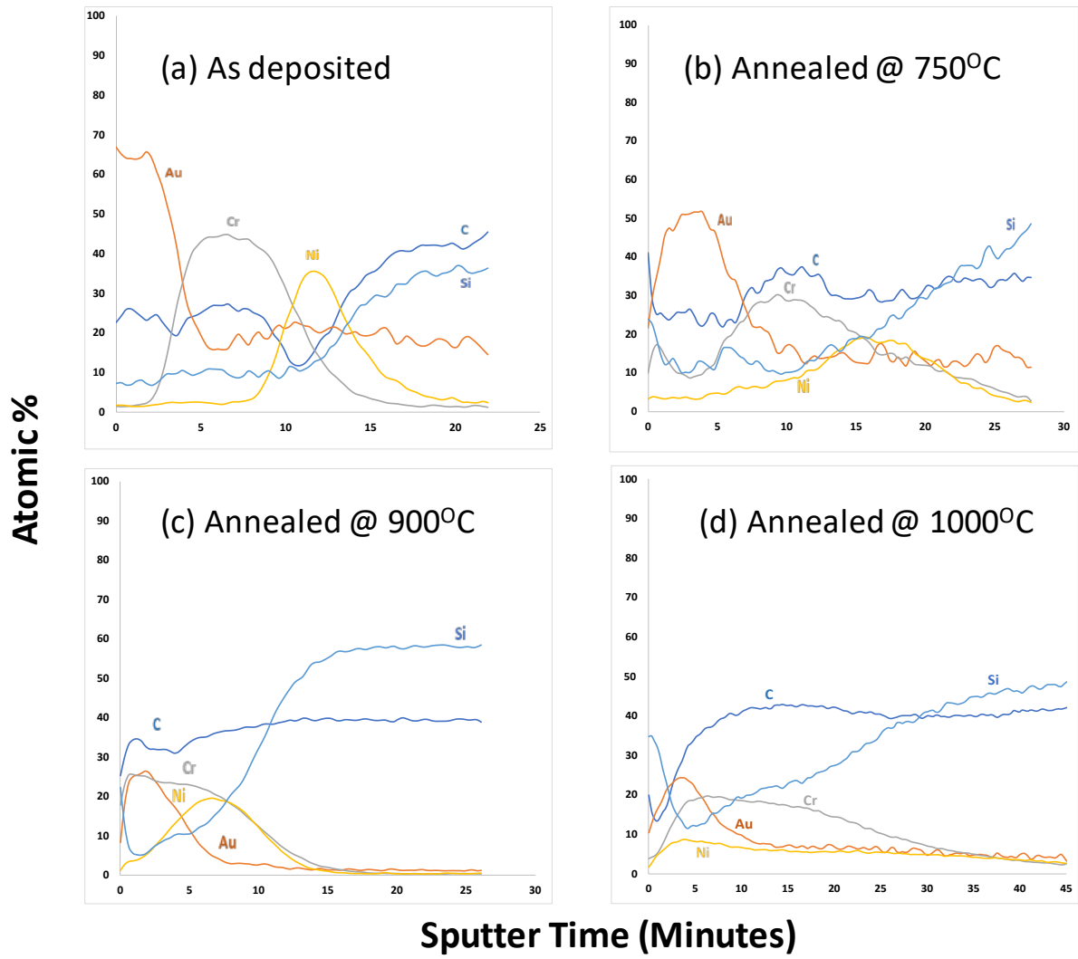
Initial AES Depth Profiles of Ohmic Contact Material 50nmAu/50nmCr/20nmNi/SiC
