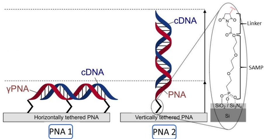
Scheme 1 Schematic illustration of PNA grafting in a horizontal (PNA 1) or vertical (PNA 2) fashion (left-hand side: red) on a Linker-activated organophosphonate monolayer (SAMP). PNA-DNA duplexes can be formed according to established Watson-Crick base pairing rules with complementary DNA (cDNA, blue).
