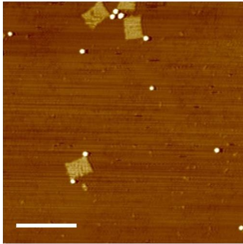
Figure 1: AFM micrograph of the DNA origami gold nanoparticles conjugates. Scale bar, 250 nm.
