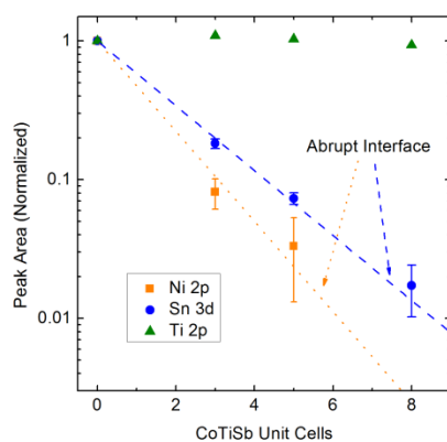
Figure 3. XPS of Peak area ratios of NiTiSn as a function of CoTiSb overlayer thickness. Dotted lines show calculated attenuation for complete coverage and abrupt interfaces
