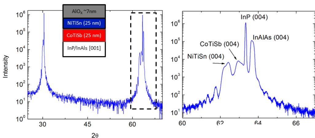
Figure 2. XRD of NiTiSn/CoTiSb on a InAlAs/InP Structure
