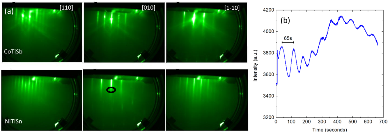
Figure 1. a) RHEED images of CoTiSb/NiTiSn on InAlAs/InP b) RHEED intensity vs time taken from the black circle in fig 1a as NiTiSn growth is initiated
