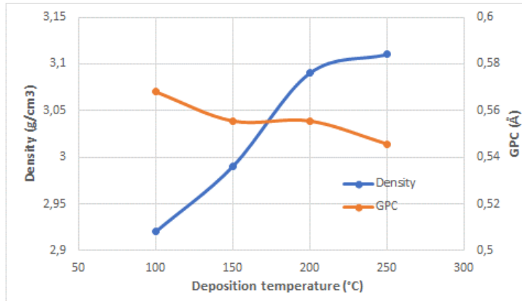
Fig. 1. AlN film density and growth per cycle as a function of deposition temperature.
