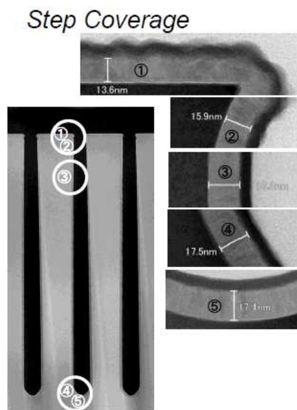
Fig. 3. Conformal step coverage (> 90 %) of AlN at AR 1:20.
