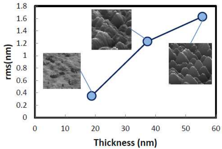
Fig. 2. AlN roughness as the film thickness increases.
