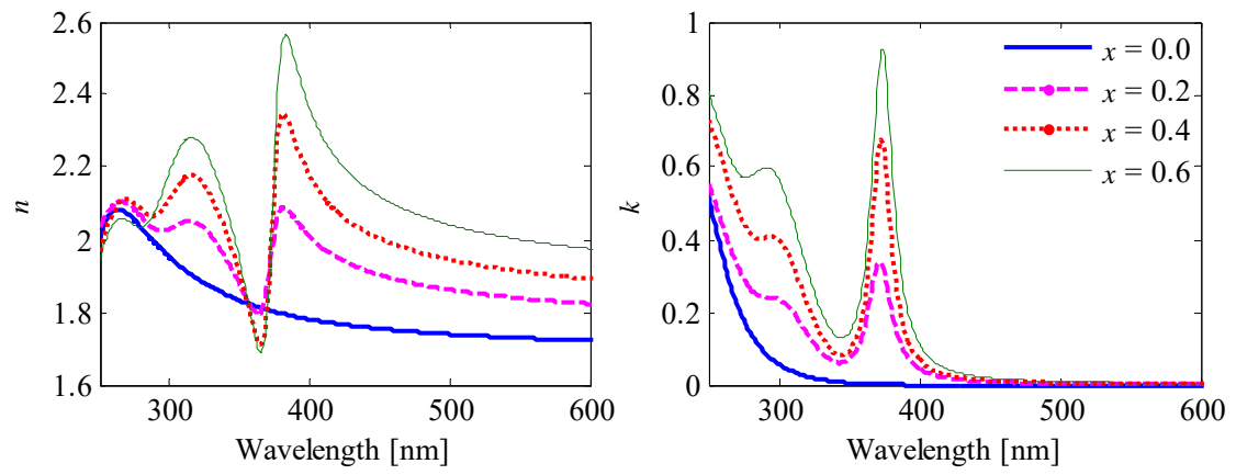
Fig. 1: Optical constants of \text{Cs}_2\text{AgIn}_{(1-x)}\text{Bi}_x\text{Cl}_6 perovskites determined by the ellipsometer.
