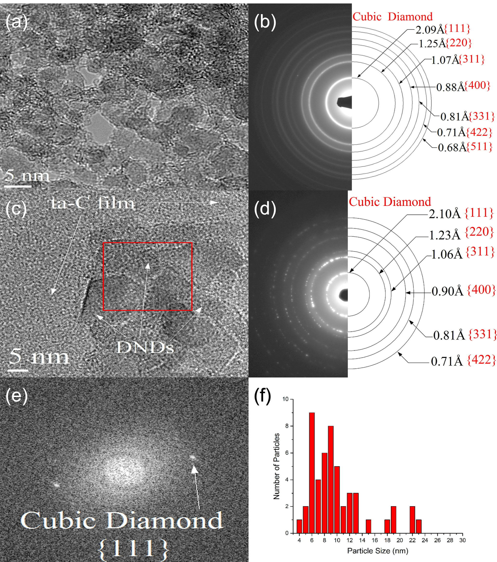
Figure caption: (a) HRTEM images of DNDs used for the composite film; (b) SAED of DNDs indicating cubic diamond phase; (c) HRTEM of DND-DLC composite film; (d) SAED of DND-DLC composite film indicating cubic diamond phase; (e) FFT of red box in (c); (f) DND particle size distribution in DND-DLC composite film estimated by HRTEM images.
