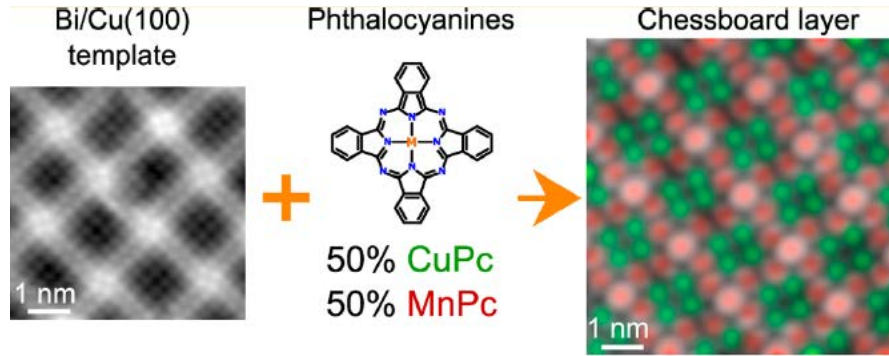
Fig1: Molecular chessboard layer containing two different metal-Pcs on Bi reconstructed Cu(100) template.
