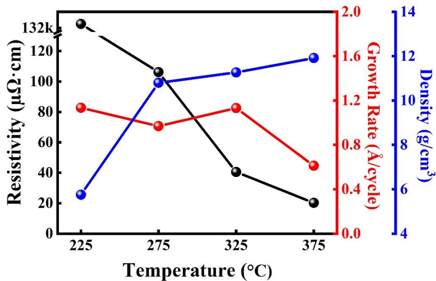
Fig. S1. Resistivity, Growth rate, and Density according to deposition temperature
