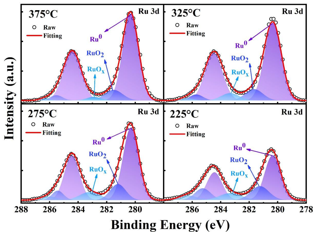
Fig. S2. XPS Analysis of Ruthenium thin films with different deposition temperature
