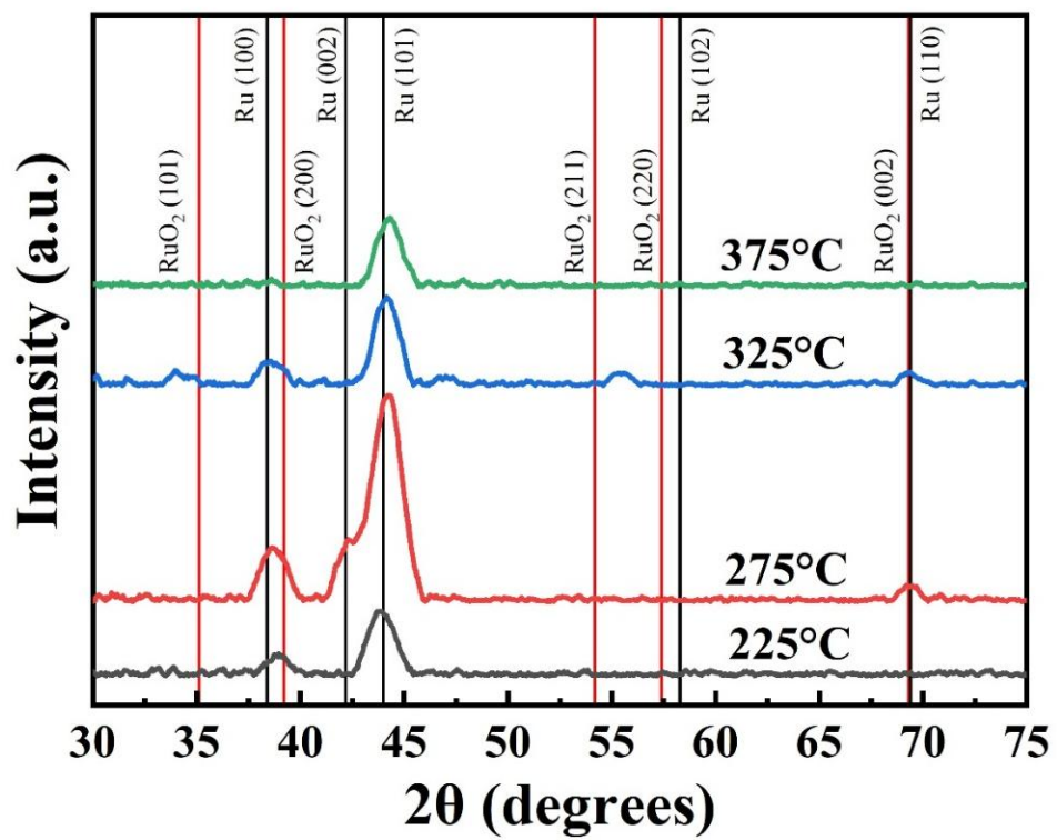
Fig. S3. XRD pattern of Ruthenium thin films with different deposition temperature
