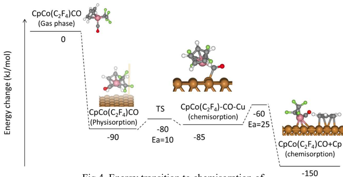
Fig.4. Energy transition to chemisorption of \text{CpCo}(\text{C}_2\text{F}_4)\text{CO} on Cu surface
