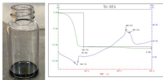
Fig.3. Vapor pressure and TG-DTA measurement results of synthesized complex: \text{CpCo}(\text{C}_2\text{F}_4)\text{CO}
