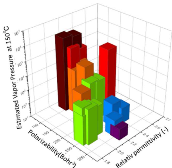
Fig.1. Vapor pressure dependencies on polarizability and relative permittivity
