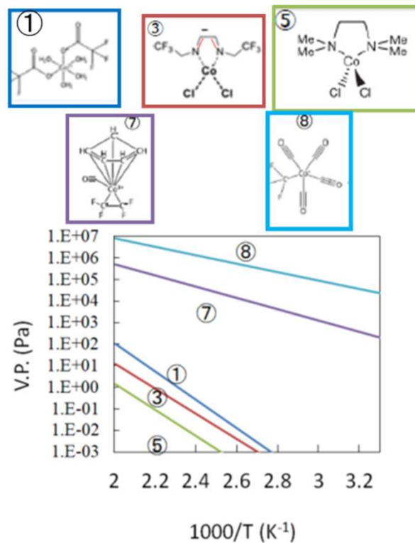
Fig.2. Estimated vapor pressure of Co-ALD precursor candidates
